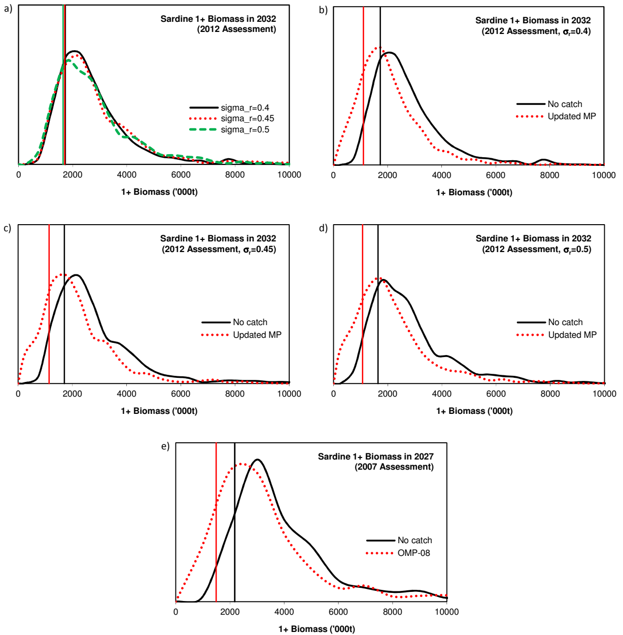
Figure 1. The projected sardine single stock 1+ biomass distribution after 20 years under a) a no catch scenario and three different underlying operating models assuming different time-invariant levels of recruitment variability, b) a no catch and MP scenario assuming \sigma_{j=1,r}^S = 0.4 , c) a no catch and MP scenario assuming \sigma_{j=1,r}^S = 0.45 , and d) a no catch and MP scenario assuming \sigma_{j=1,r}^S = 0.5 . The 20%iles of the distributions are shown by the dashed vertical lines. The projected distributions simulated under OMP-08 and a no catch scenario using the 2007 assessment (using samples from distributions assuming \sigma_{j=1,r}^S = 0.4 , \sigma_{j=1,r}^S = 0.5 , \sigma_{j=1,r}^S = 0.6 and \sigma_{j=1,r}^S = 0.7 ) is shown in e) for comparison.
